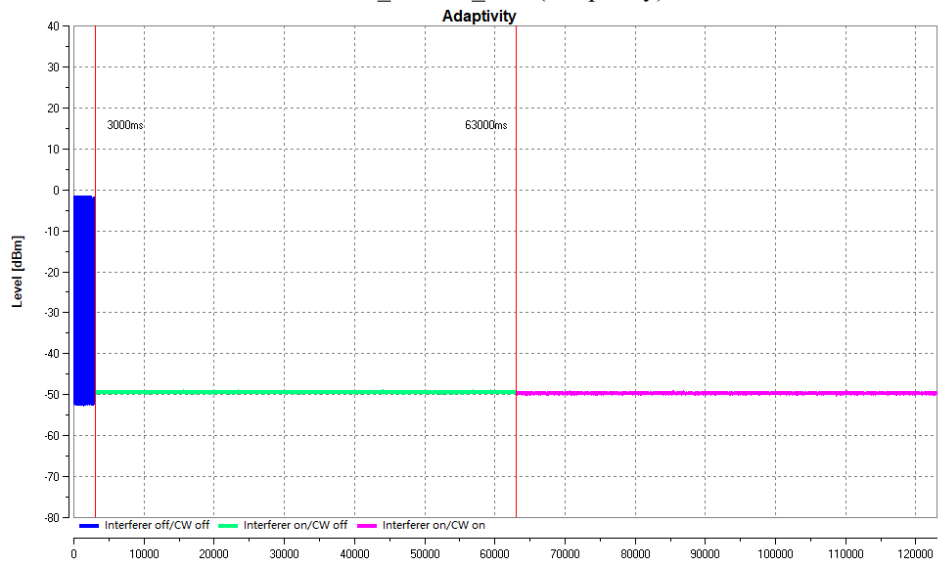
802.11b_Chain 0_2472(Adaptivity)
