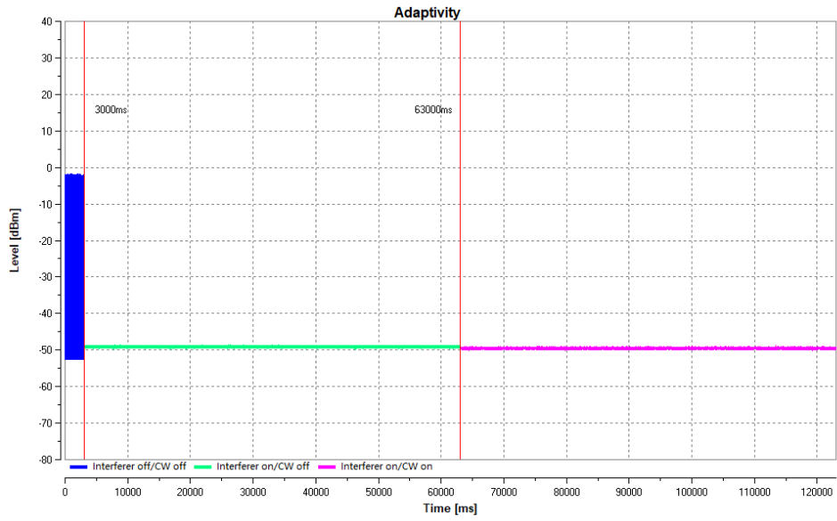
802.11b_Chain 0_2472(Adaptivity)
