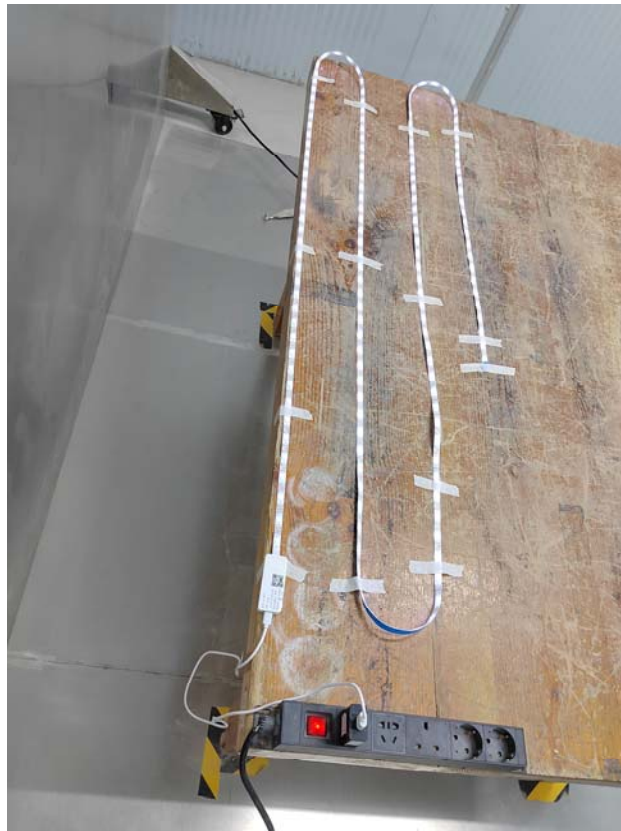
Conducted Emissions Side View-Model: L3-5M-P
