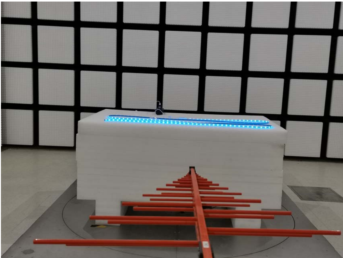
Radiated Emission Below 1GHz View-Model: L3-5M
