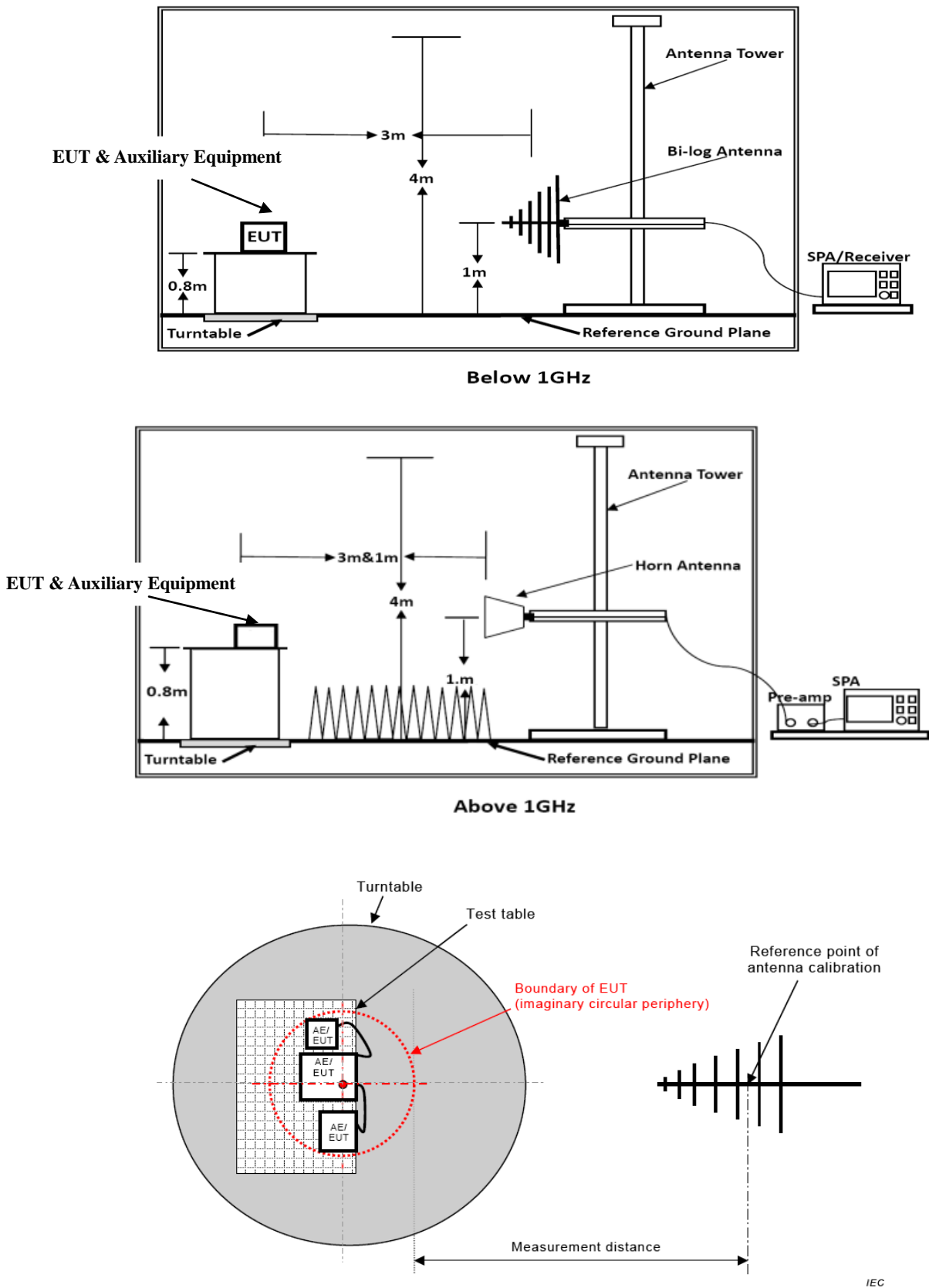
Figure C.1 – Measurement distance
